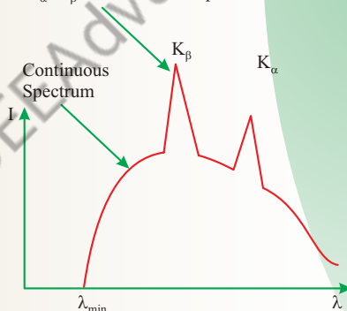
K_{\alpha} - K_{\beta} -Characteristic Spectrum
